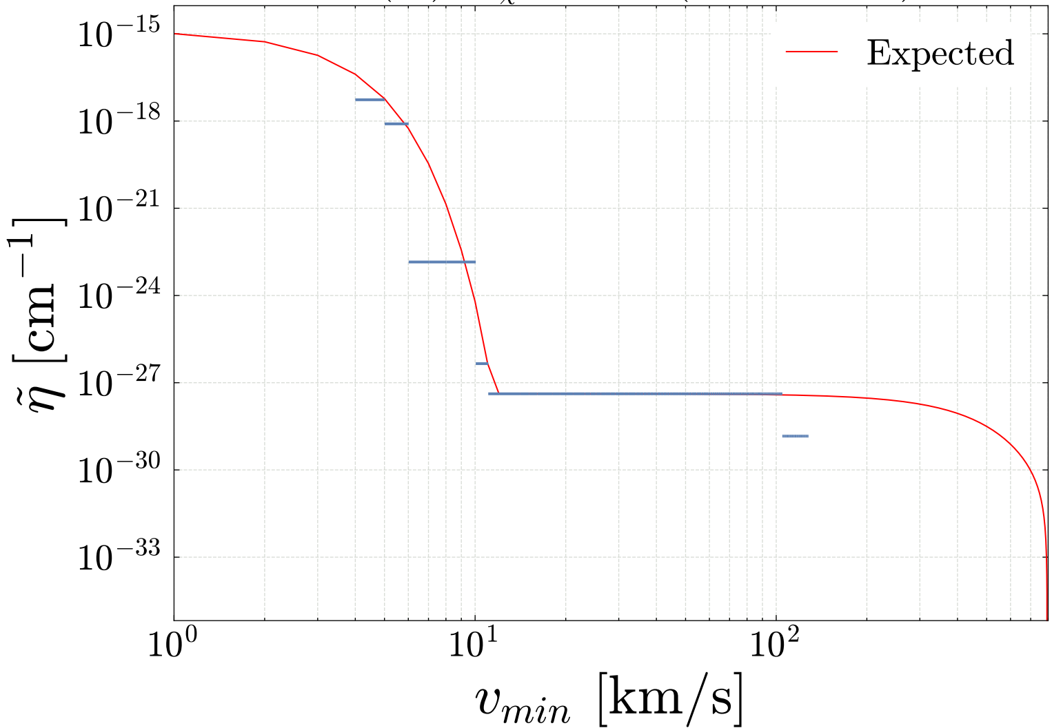
TES(Al): m_\chi = 1 GeV (Earth-Bound)
