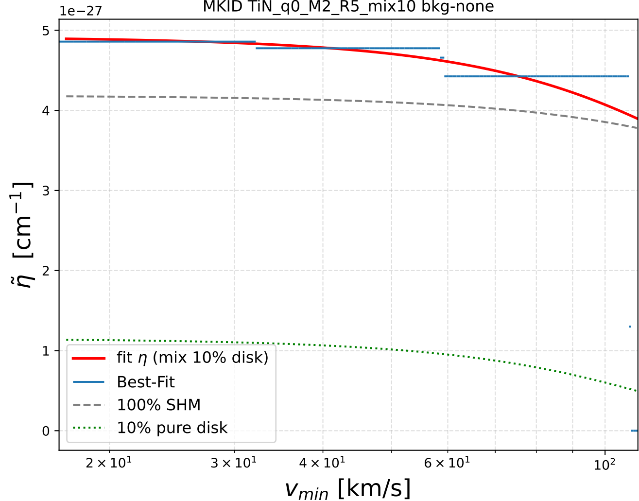
MKID TiN_q0_M2_R5_mix10 bkg-none
