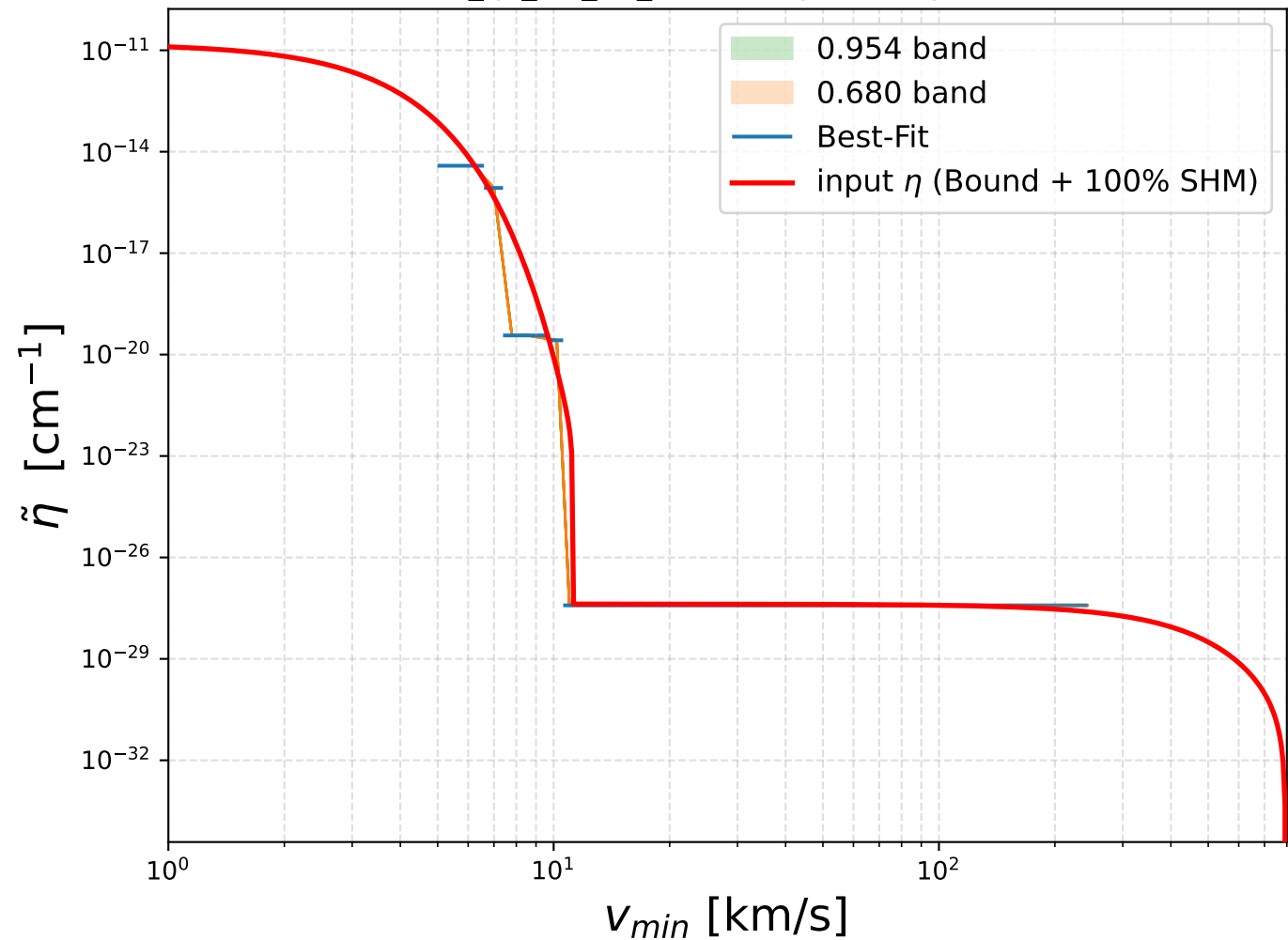
MKID TiN_q0_M3_R5_Bound bkg-none (profile band)
