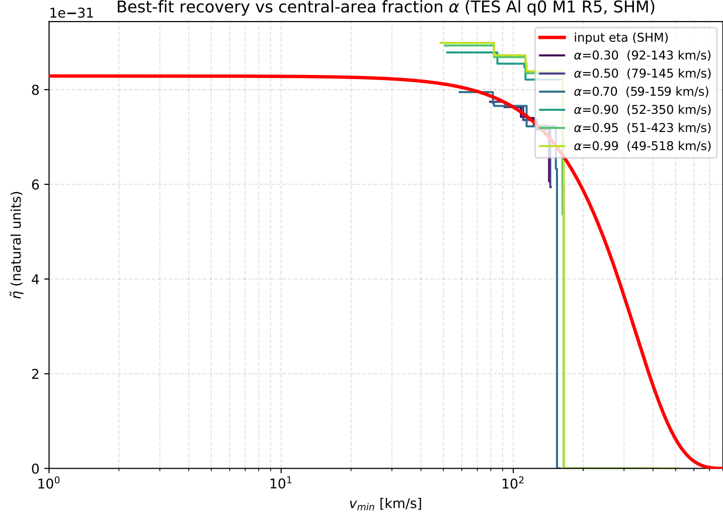
Best-fit recovery vs central-area fraction \alpha (TES A1 q0 M1 R5, SHM)
