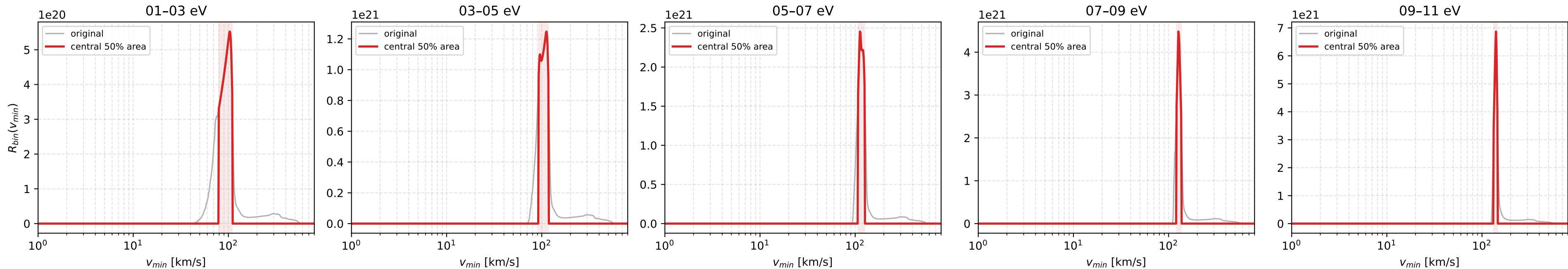
Response functions: original vs central-50%-area cut (TES Al q0 M1 R5)
