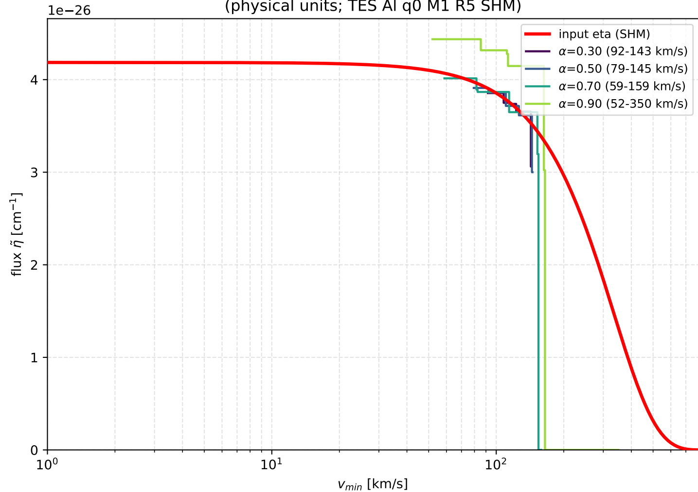
Central-area alpha sweep, full no-band-aid pipeline at GeV=1e42 (physical units; TES Al q0 M1 R5 SHM)
