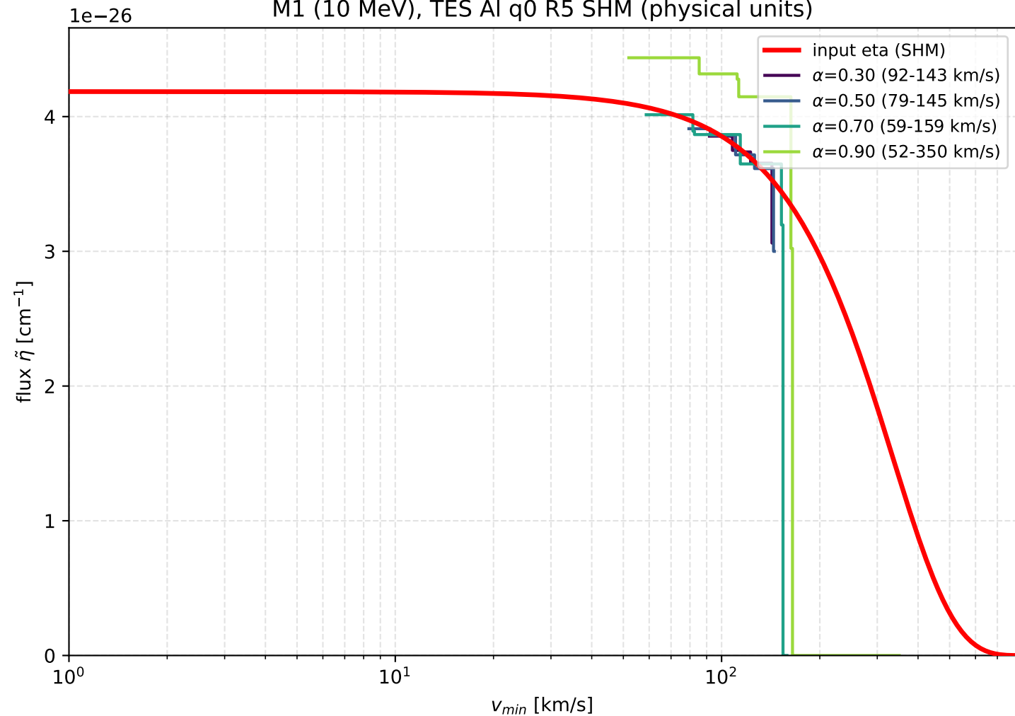
Central-area alpha sweep, no-band-aid pipeline at GeV=1e42 M1 (10 MeV), TES Al q0 R5 SHM (physical units)
