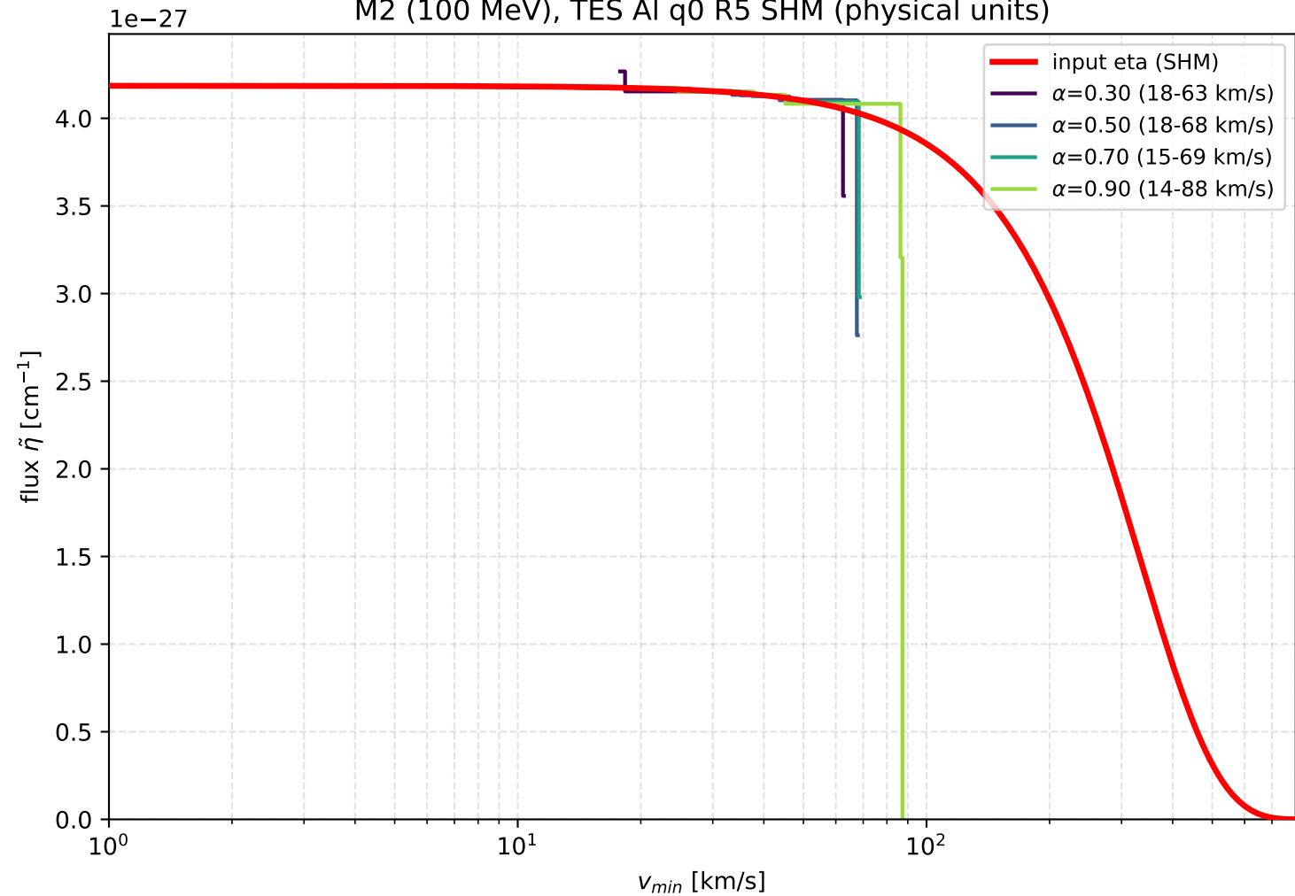
Central-area alpha sweep, no-band-aid pipeline at GeV=1e42 M2 (100 MeV), TES Al q0 R5 SHM (physical units)
