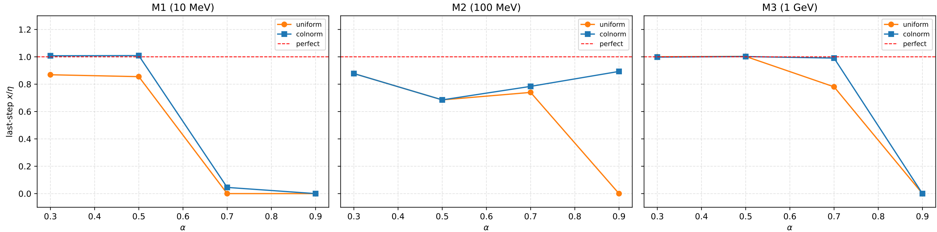
colnorm vs uniform last-step recovery -- TES (AI) q0 R5 SHM
