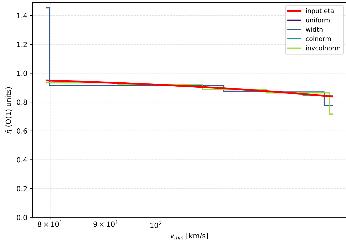
Minimal-flux objective weighting, M1 (10 MeV), alpha=0.5
