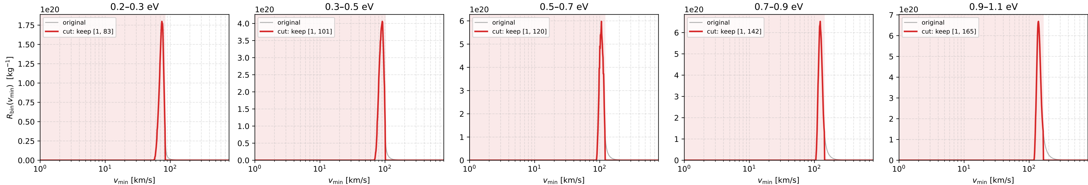
TiN_q0M1_R5 (M1): response functions, original vs cut (high-v cut at 20% of peak value, low side kept)
