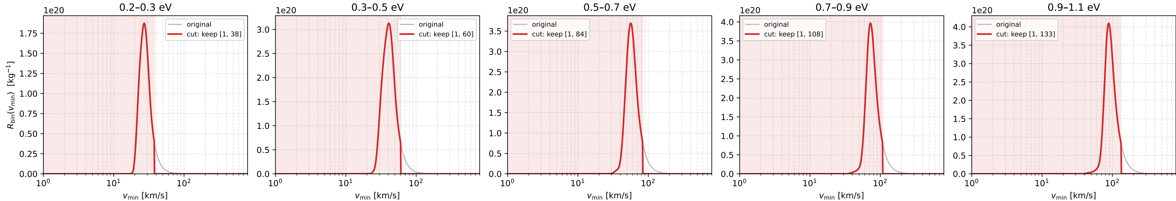
TiN_q0M2_R5 (M2): response functions, original vs cut (high-v cut at 20% of peak value, low side kept)
