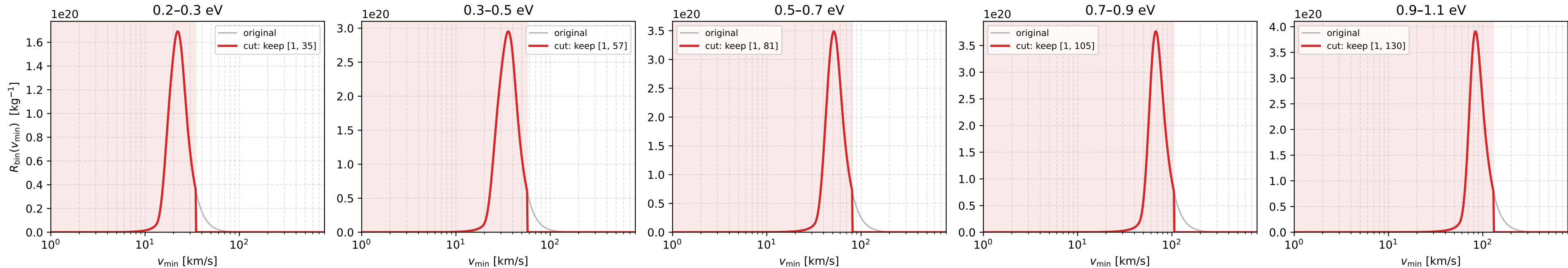
TiN_q0M3_R5 (M3): response functions, original vs cut (high-v cut at 20% of peak value, low side kept)
