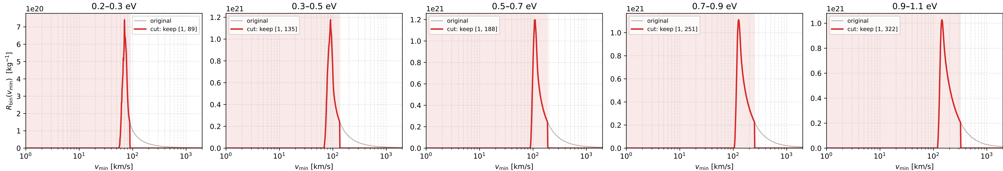
TiN_q2M1_R5 (M1): response functions, original vs cut (high-v cut at 20% of peak value, low side kept)
