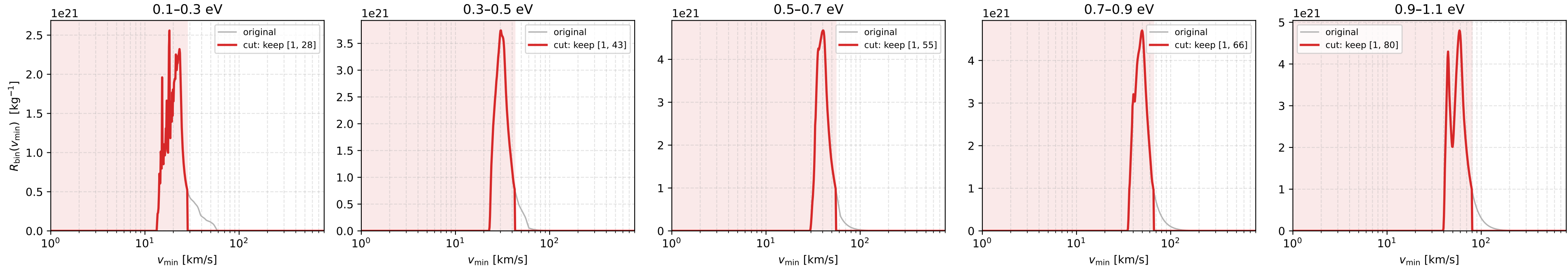
Al_q0M2_R5 (M2): response functions, original vs cut (high-v cut at 20% of peak value, low side kept)
