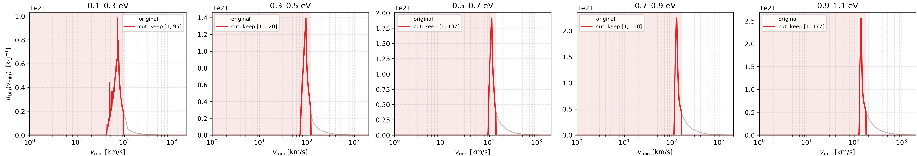
Al_q2M1_R5 (M1): response functions, original vs cut (high-v cut at 20% of peak value, low side kept)
