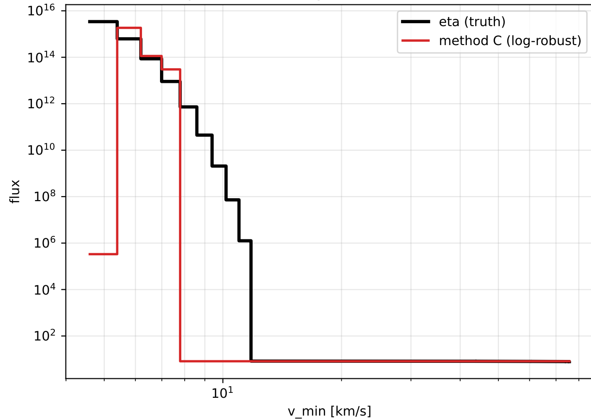
Al q0 M3 Bound (log10-RMS err=2.26 dex)
