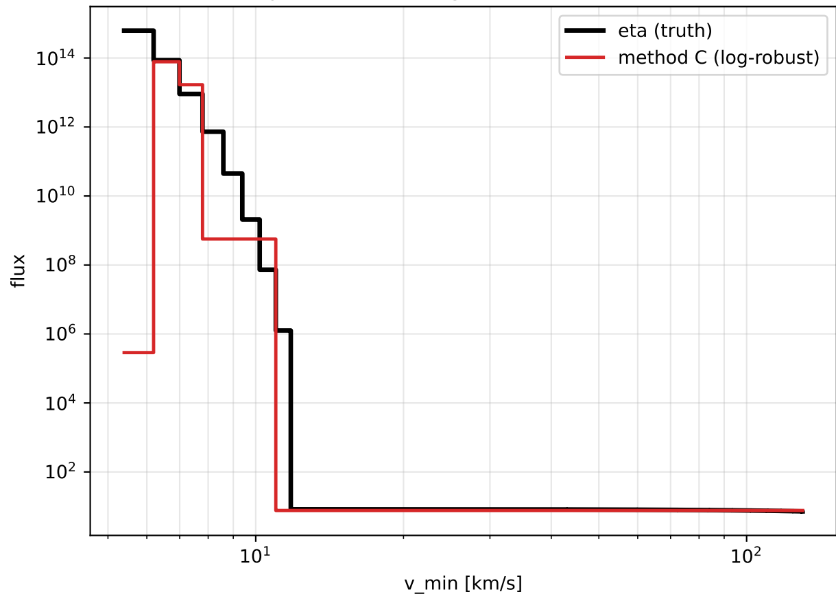
TiN q0 M3 Bound (log10-RMS err=0.91 dex)
