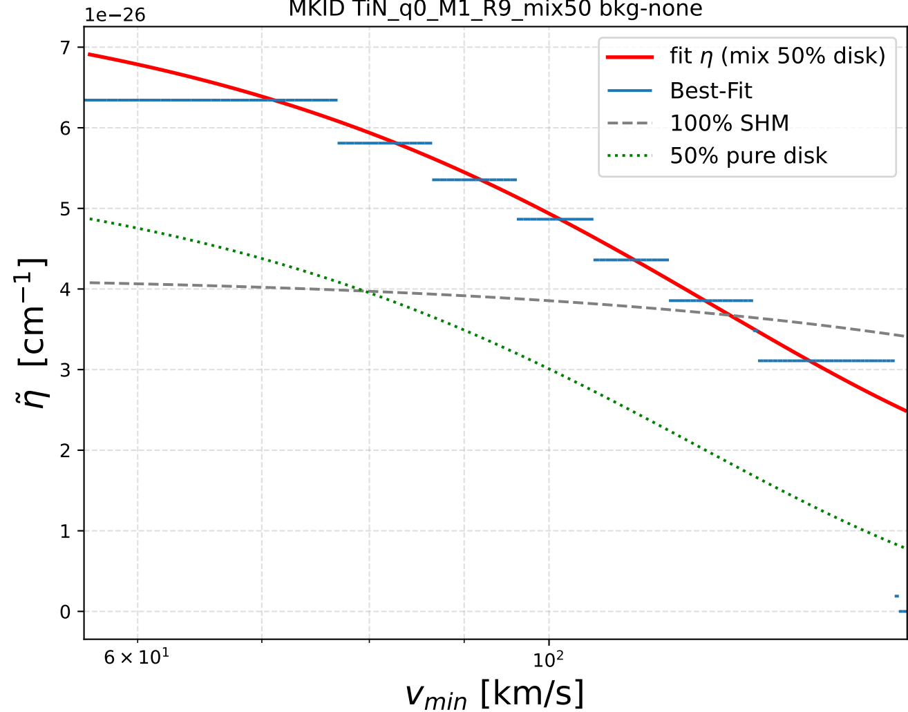
MKID TiN_q0_M1_R9_mix50 bkg-none
