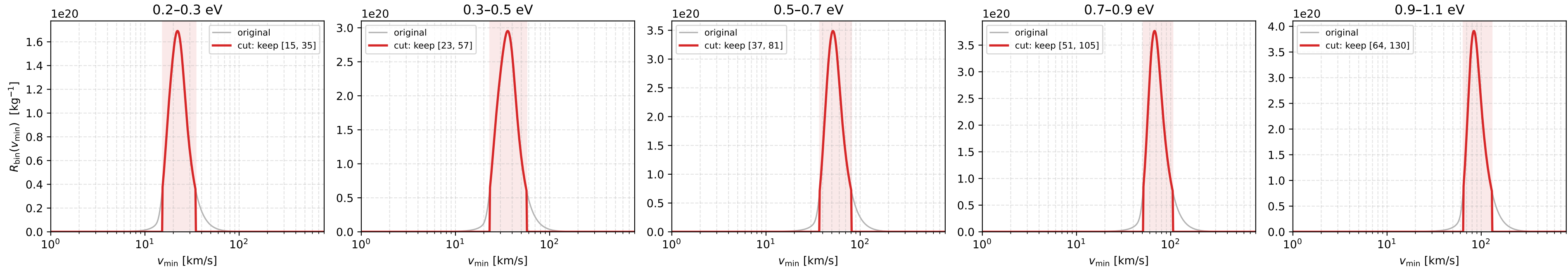
TiN_q0M3_R5 (M3): response functions, original vs cut (both-side cut at 20% of peak value)
