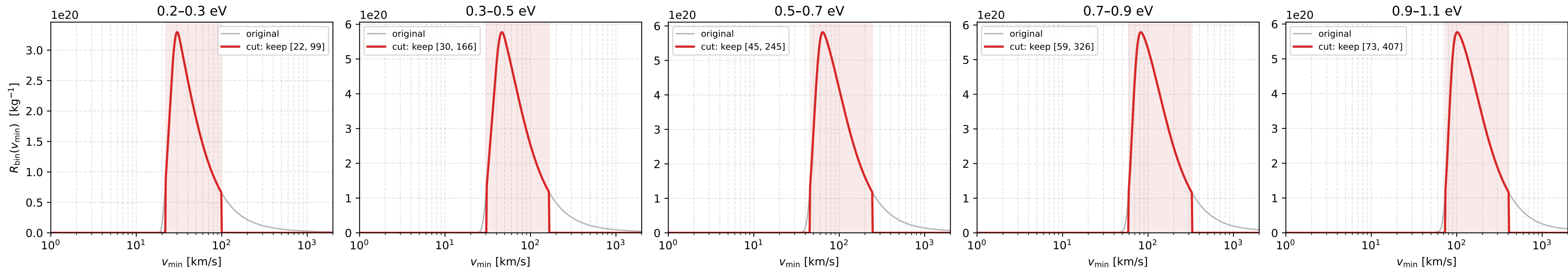
TiN_q2M2_R5 (M2): response functions, original vs cut (both-side cut at 20% of peak value)
