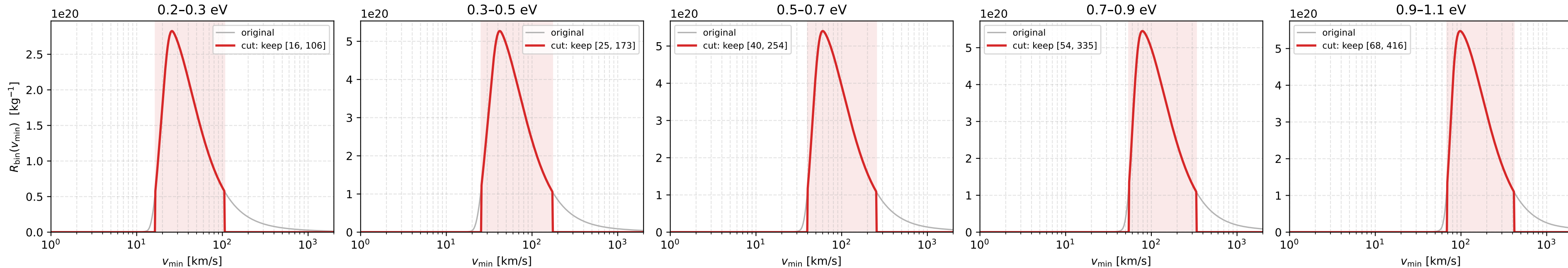
TiN_q2M3_R5 (M3): response functions, original vs cut (both-side cut at 20% of peak value)
