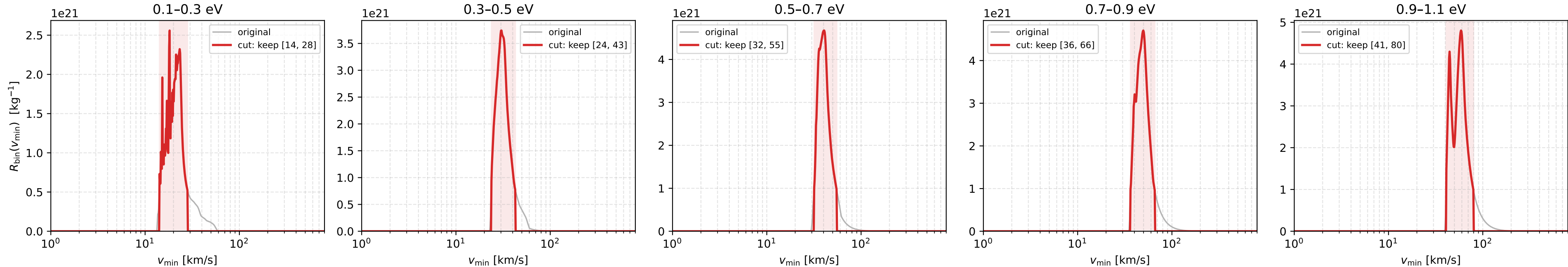
Al_q0M2_R5 (M2): response functions, original vs cut (both-side cut at 20% of peak value)
