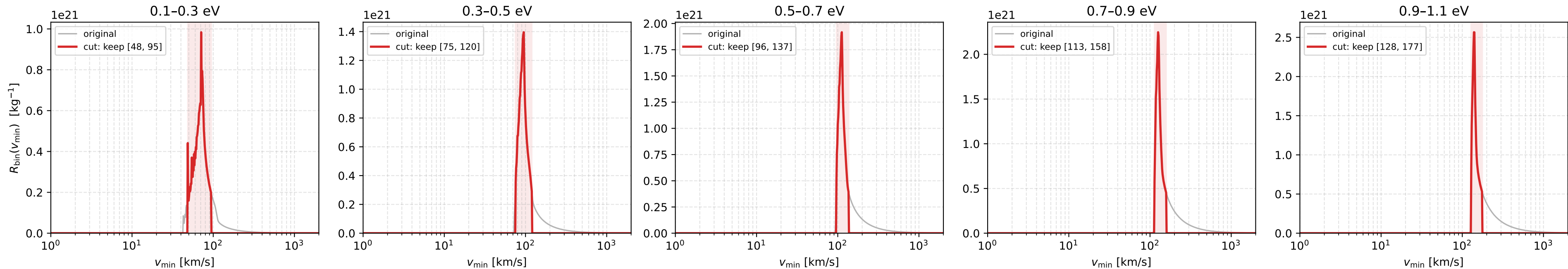
Al_q2M1_R5 (M1): response functions, original vs cut (both-side cut at 20% of peak value)
