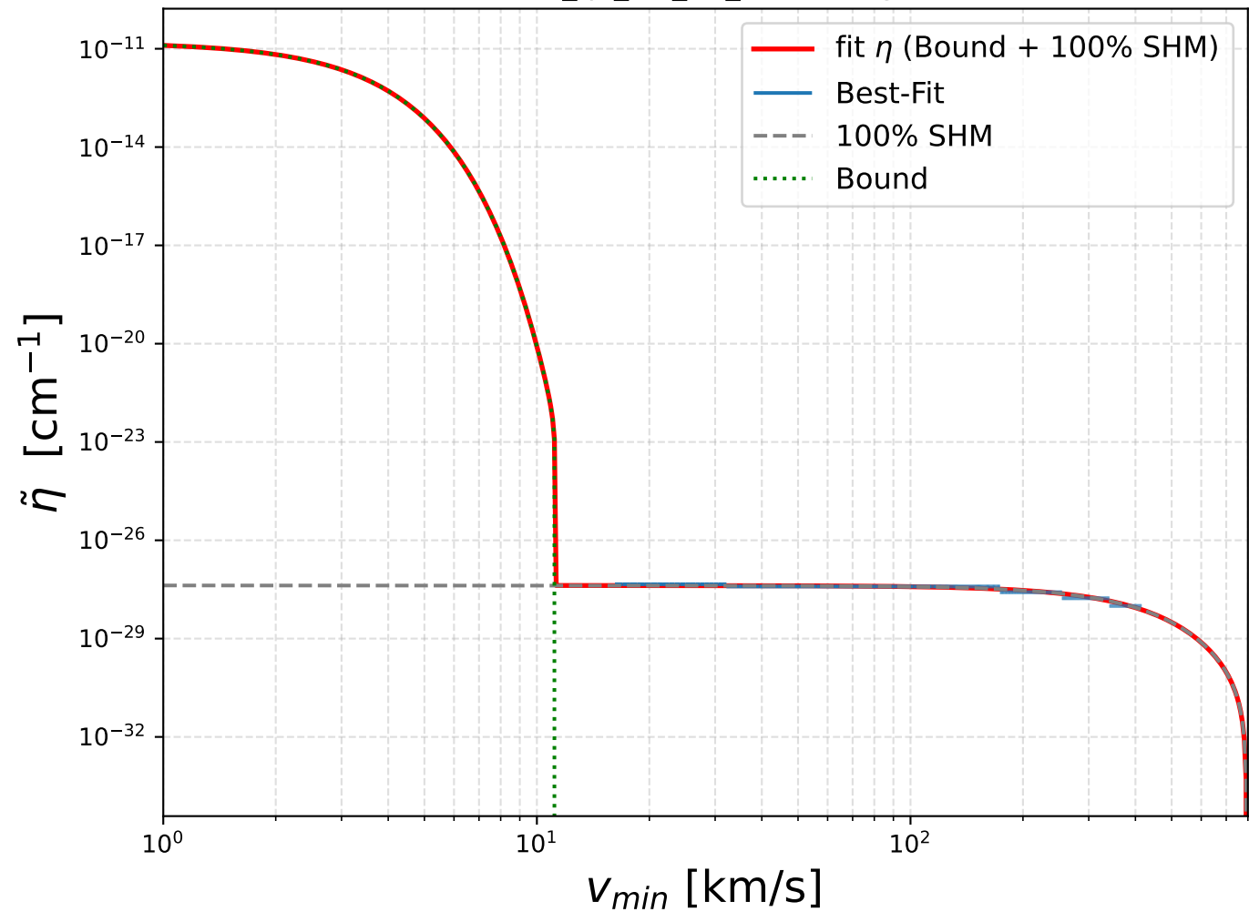
MKID TiN_q2_M3_R5_Bound bkg-none
