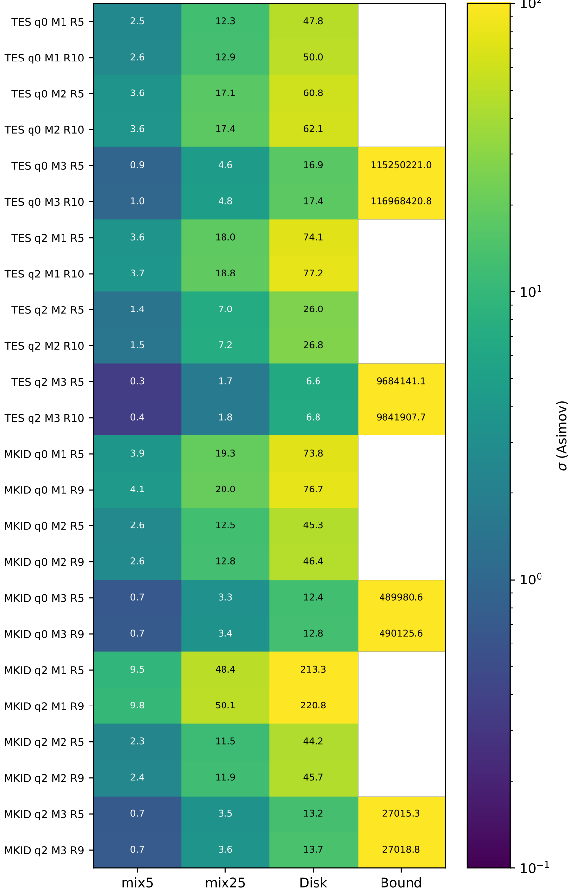
Median discrimination significance vs Halo [ \sigma ], bkg-b
