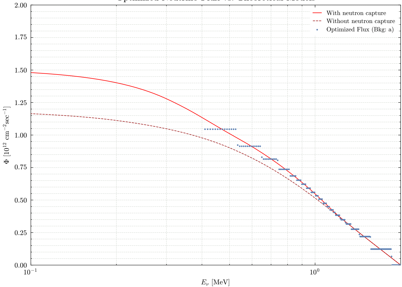
Optimized Neutrino Flux vs. Theoretical Models
