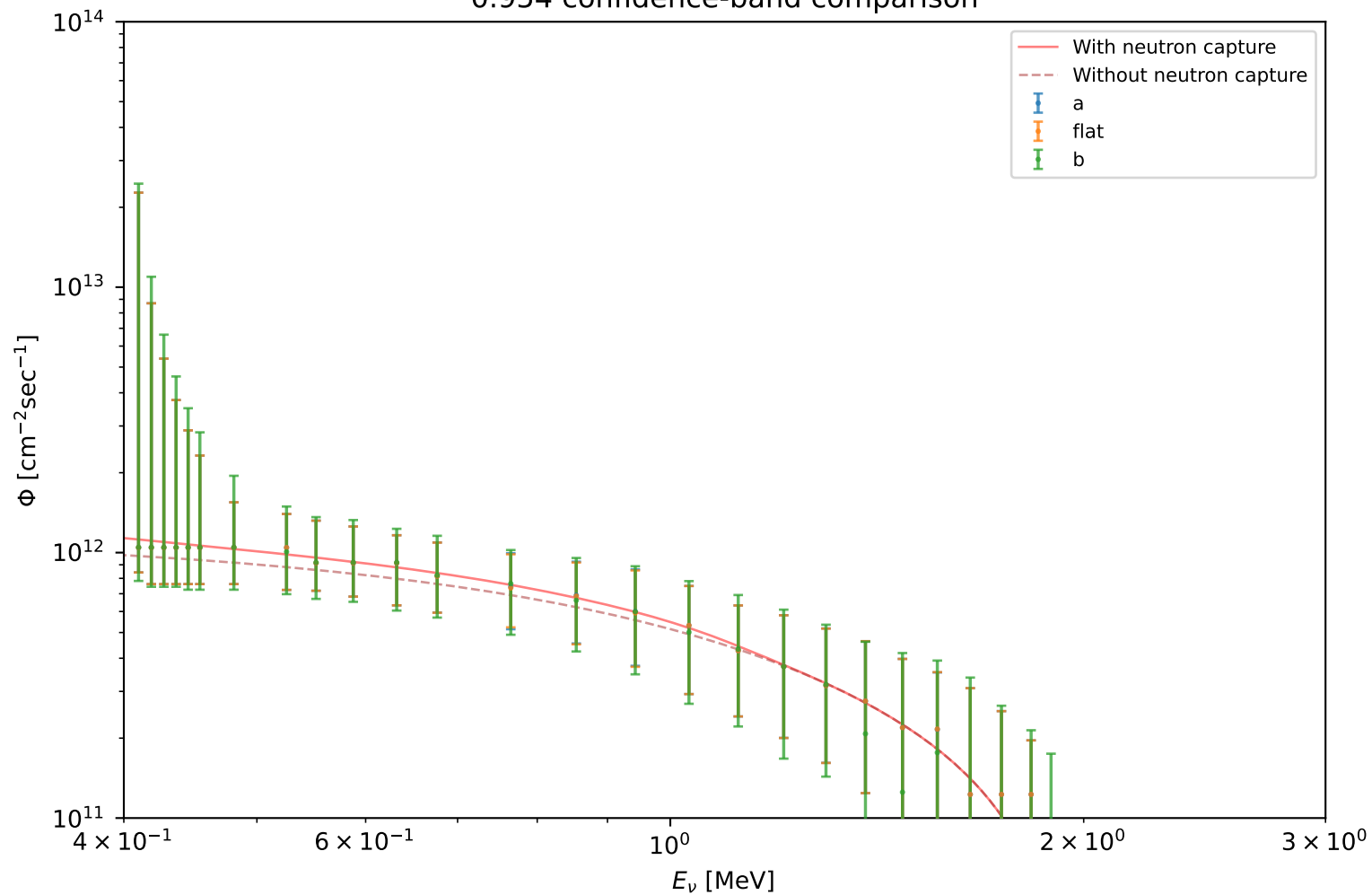
0.954 confidence-band comparison
