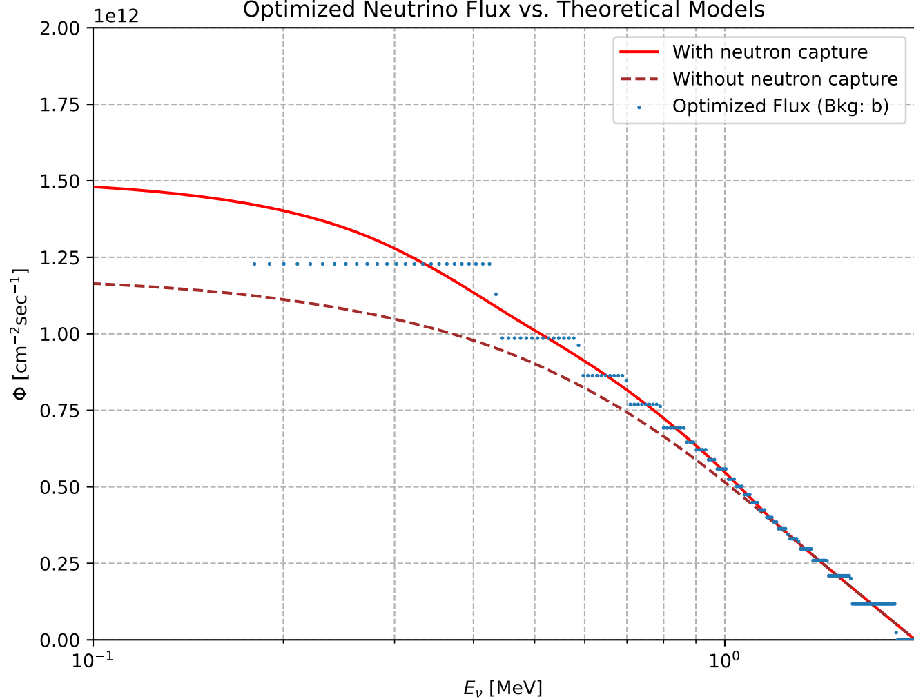
Optimized Neutrino Flux vs. Theoretical Models
