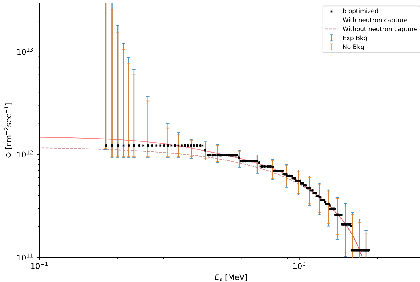
0.954 confidence-band comparison
