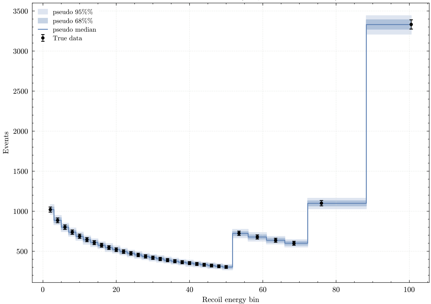
Pseudo-data vs. true data (Bkg: a, T=3, N=500)
