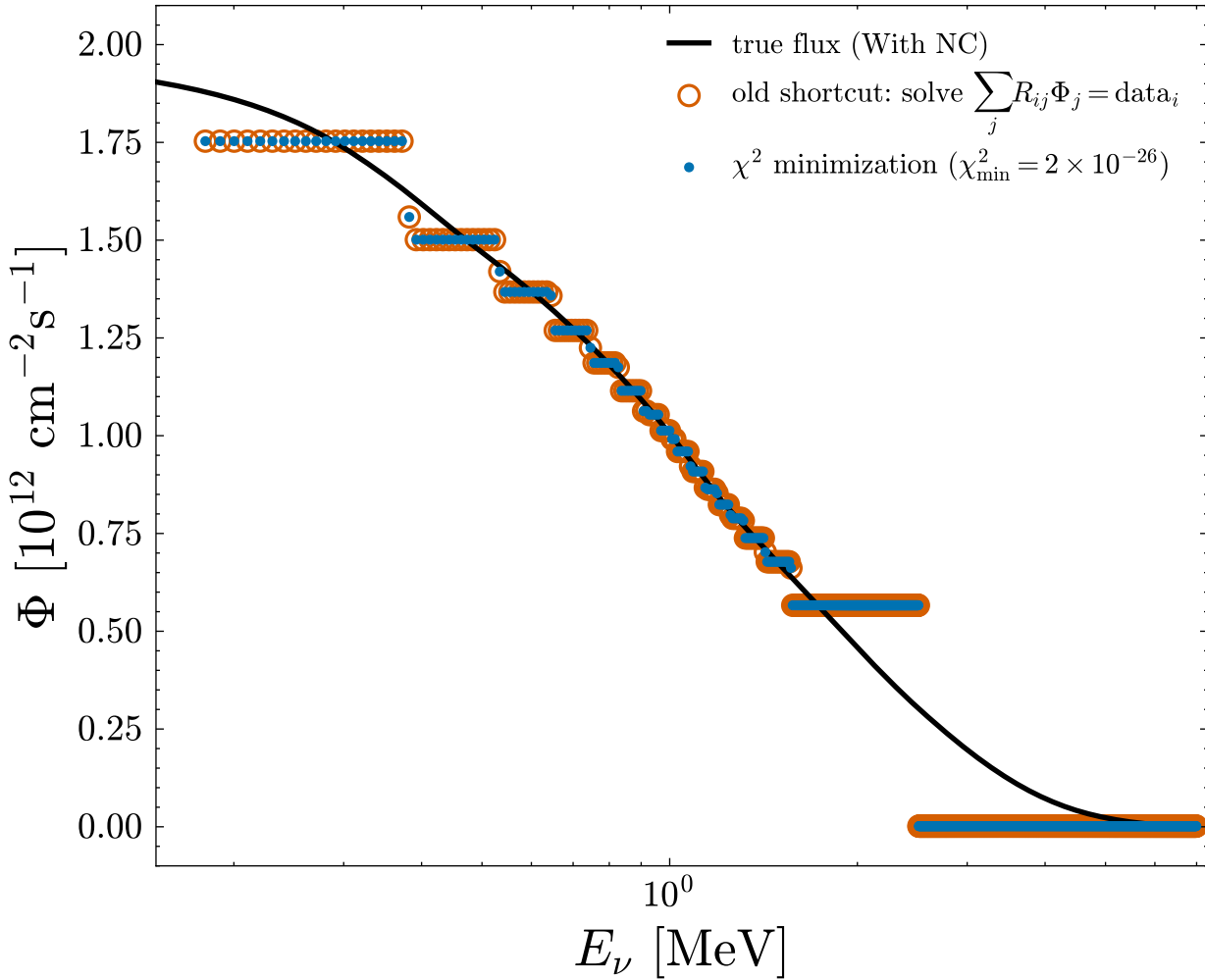
(a) E'_{\text{thr}} = 1 eV: max difference / \Phi(E_{\text{min}}) = 4\text{e-}12
