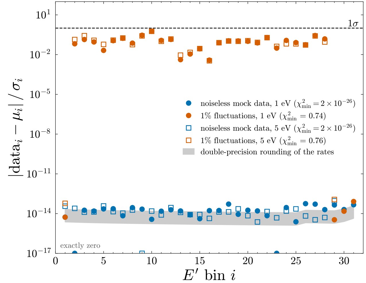
(c) residual per bin of the \chi^2 minimization
