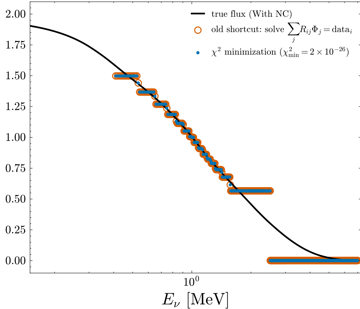
(b) E'_{\text{thr}} = 5 eV: max difference / \Phi(E_{\text{min}}) = 2\text{e-}11
