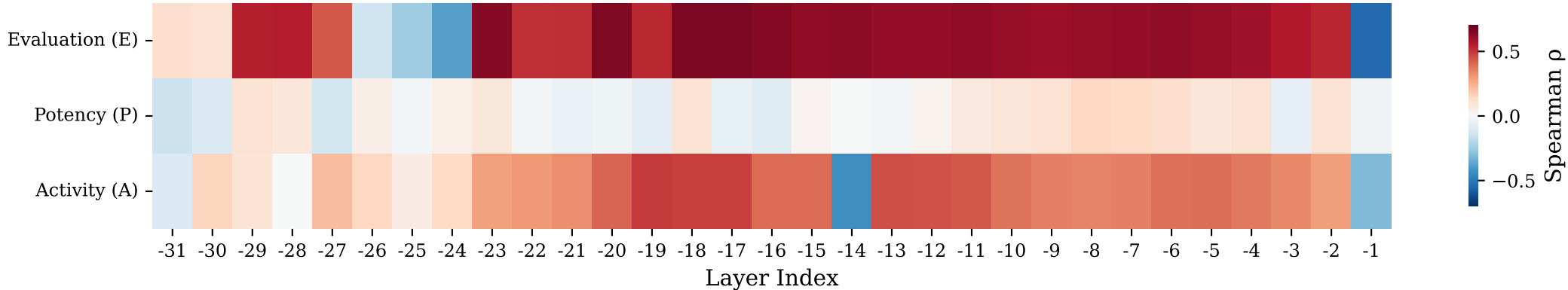
Per-Layer Reading Correlation with Ground-Truth EPA
