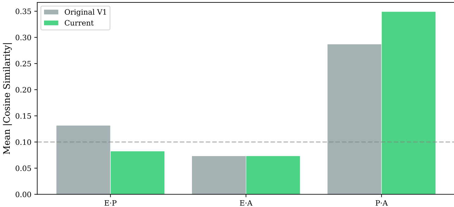
Cross-Dimension Entanglement by Direction Set
