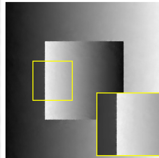
U-Tikhonov 42.16 dB / 0.9874
