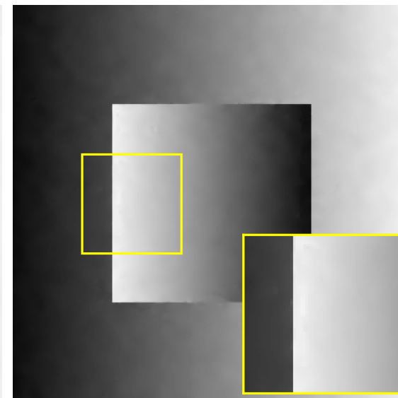
U-TGV 42.87 dB / 0.9855
