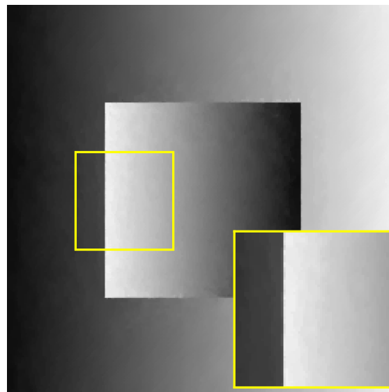
U-TV 41.79 dB / 0.9840
