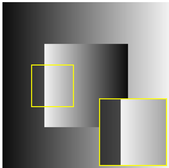
Clean Reference
