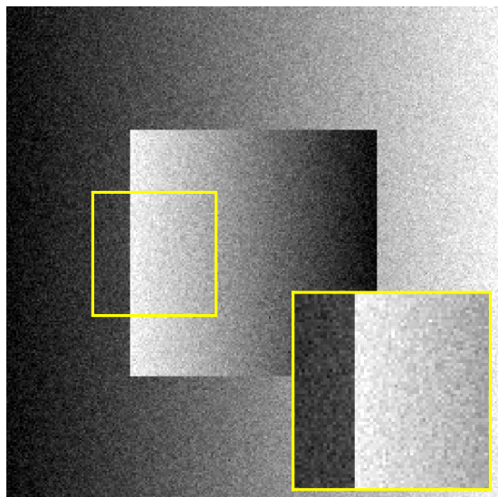
Noisy 26.12 dB / 0.4357
