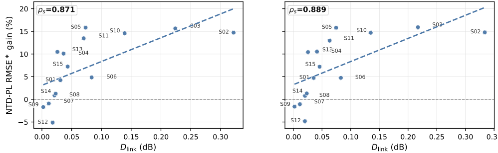
Figure 7: Scene-level supplement for the CAVE completion diagnostic table. The left and right panels use missing rates 0.3 and 0.5, respectively; D_{\text{link}} from frozen-backbone Link Refresh predicts larger held-out RMSE* gains.
