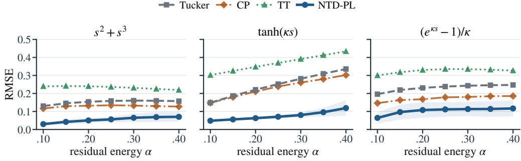
Figure 1: Controlled nonlinear residual sweep. NTD-PL stays Tucker-like near the linear regime and separates as \alpha , the nonlinear residual energy, increases. Lower RMSE is better.
