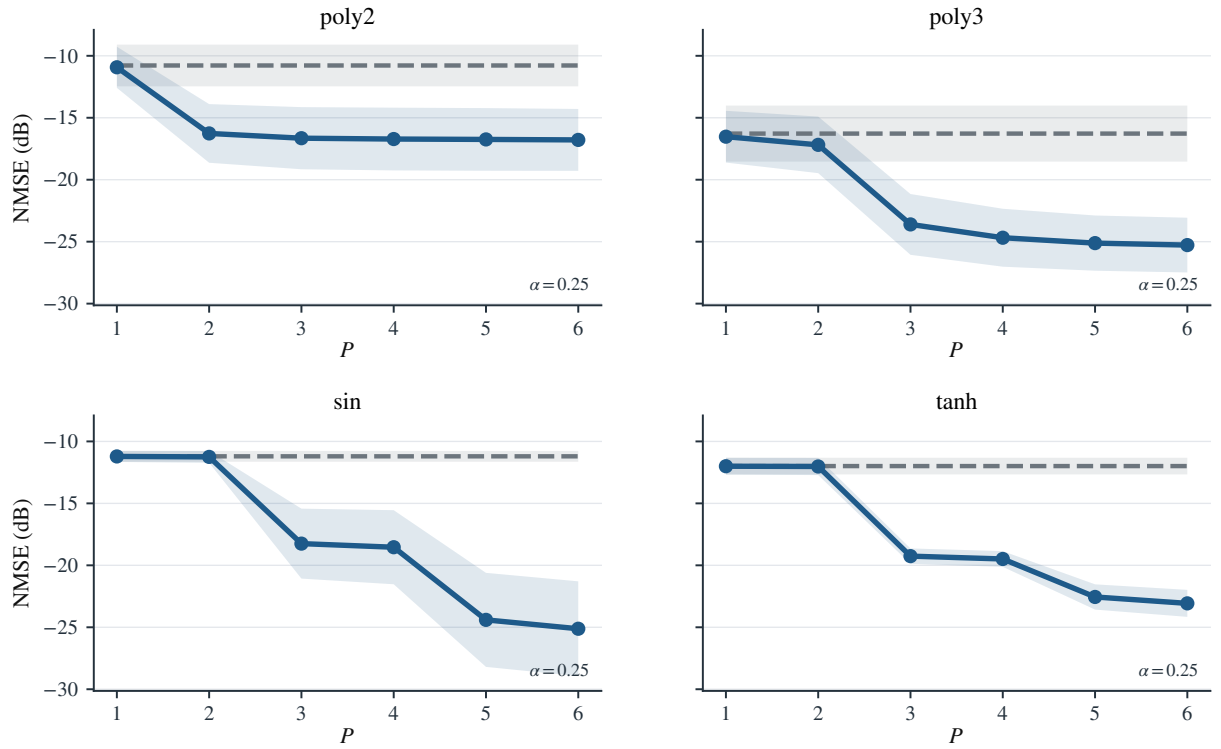
Figure 2: Variation of the approximation error of NTD-PL with the maximum polynomial degree P under a fixed nonlinear strength, together with Tucker as a reference; the gray horizontal line indicates the Tucker baseline. The figure shows that P = 1 is close to Tucker, confirming linear consistency, and that the error decreases as P increases, with gradually saturating marginal gains.
