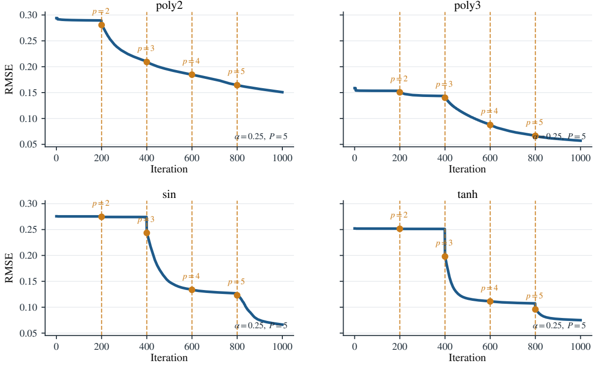
Figure 3: Training-loss curves of NTD-PL under the progressive degree-increasing strategy. The dashed lines mark the degree-switching milestones, and most cases show a stage-wise drop after each increment, indicating that newly activated orders absorb previously unmodeled nonlinear residuals.
