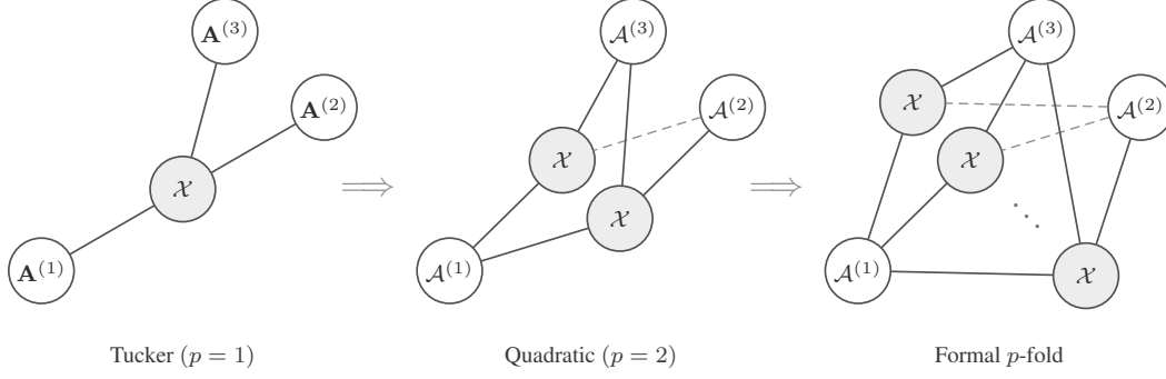
Figure 5: Tensor-network view of a formal p -fold Tucker extension. The construction keeps the Tucker idea of mode-wise generation, but lets each mode projection couple multiple latent index tuples.
