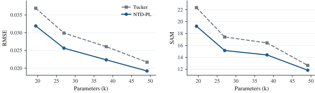
Figure 3: CAVE full-observation reconstruction as a representation-capacity check. Each point averages 15 scenes at a matched Tucker backbone rank. Unlike masked completion in Table 1, this plot measures how much error each parameter budget can represent when all entries are observed.
