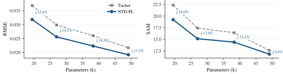
Fig. 5. CAVE full reconstruction at matched Tucker rank. NTD-PL improves both RMSE and SAM, and the gap decreases as Tucker rank increases.
