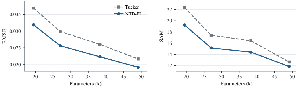
Figure 3: CAVE full reconstruction as a representation-capacity check. At matched Tucker backbone rank, NTD-PL reduces RMSE and SAM; the gap shrinks as Tucker rank increases, consistent with fixed-rank enhancement. Each point averages 15 scenes.
