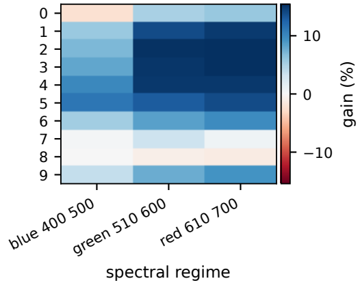
Joint regimes
