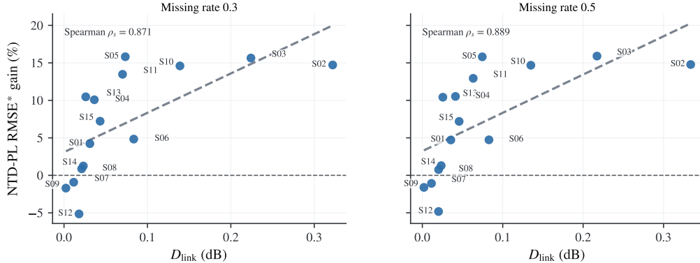
Figure 4: CAVE completion diagnostic. Scene-level D_{\text{link}} from frozen-backbone Link Refresh predicts larger held-out RMSE* gains at missing rates 0.3 and 0.5; panels annotate Spearman correlations.
