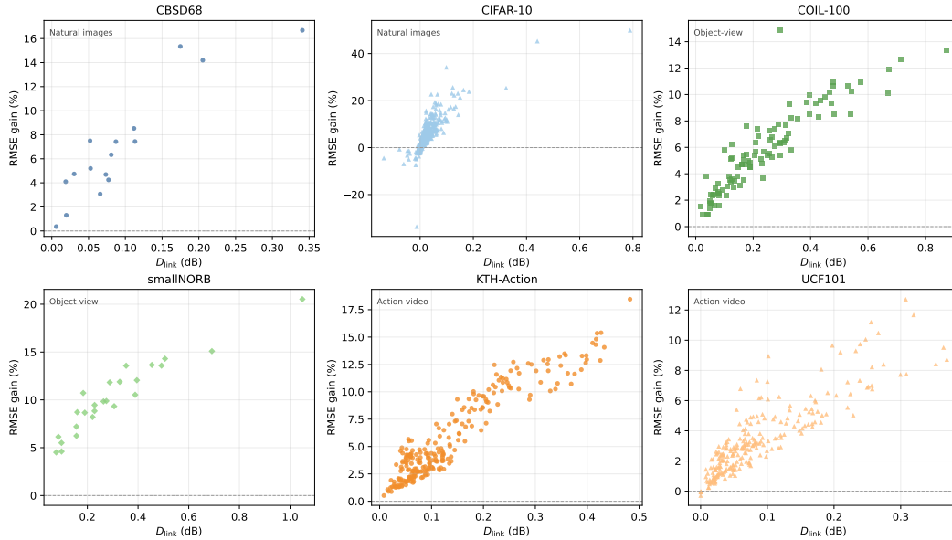
Figure 8: Per-unit non-HSI diagnostic correlation. D_{\text{link}} from frozen-backbone Link Refresh is plotted against NTD-PL RMSE gain for natural-image, object-view, and action-video units; labels are assigned from D_{\text{link}} , not from NTD-PL gain.
