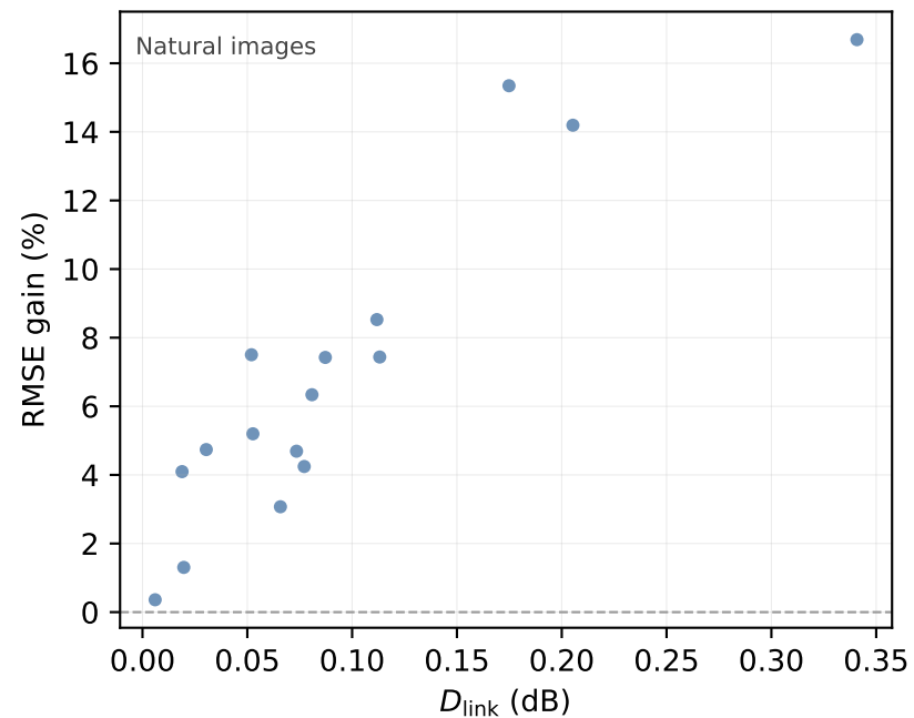
smallINORB
