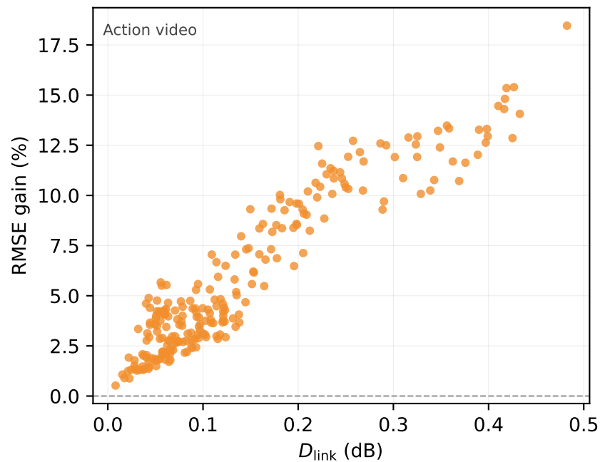
KTH-Action
