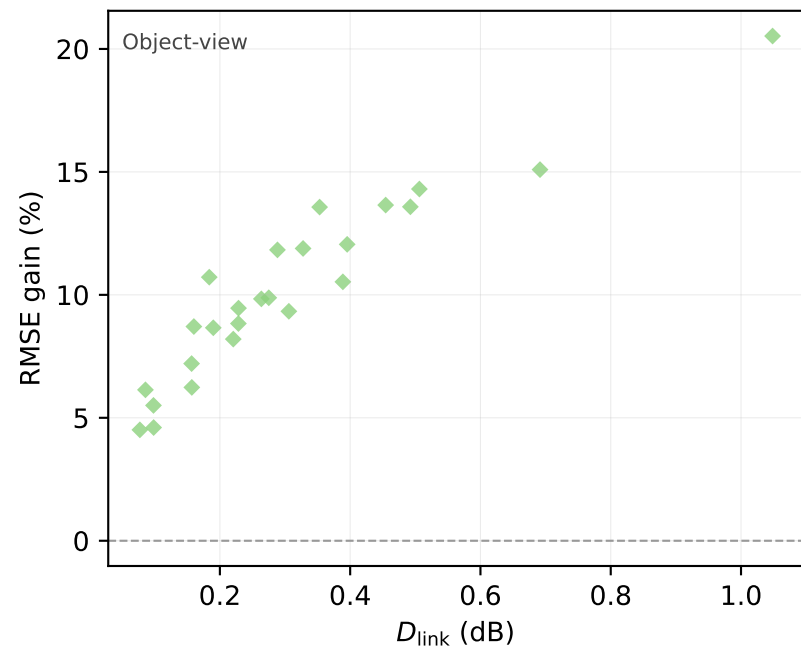
smallINORB
