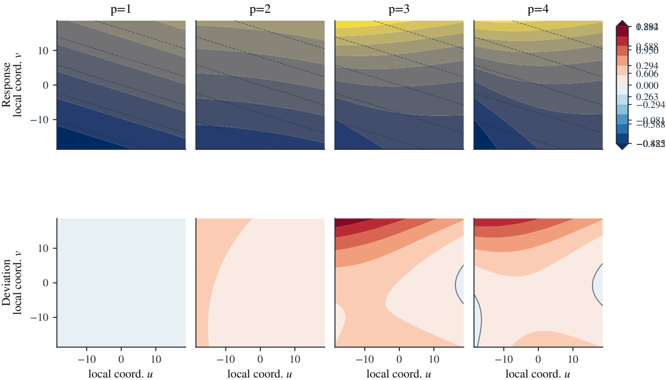
Fixed Tucker patch under the learned \beta schedule ( \alpha=0.3 )
