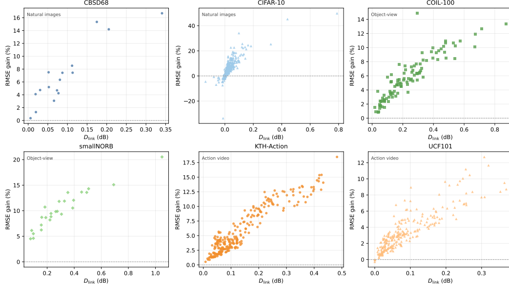
Figure 4: Per-unit non-HSI diagnostic correlation. Each panel plots D_{\text{link}} against NTD-PL RMSE gain over independently fitted tensor units. D_{\text{link}} is computed by frozen-backbone Link Refresh, and diagnostic labels are assigned from D_{\text{link}} , not from NTD-PL gain. The figure shows domain-dependent but positive diagnostic structure.
