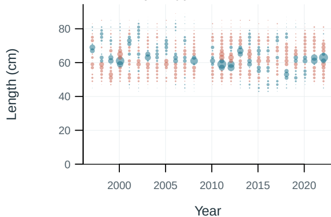
TR.INDEX.1ef.NZ-troll
