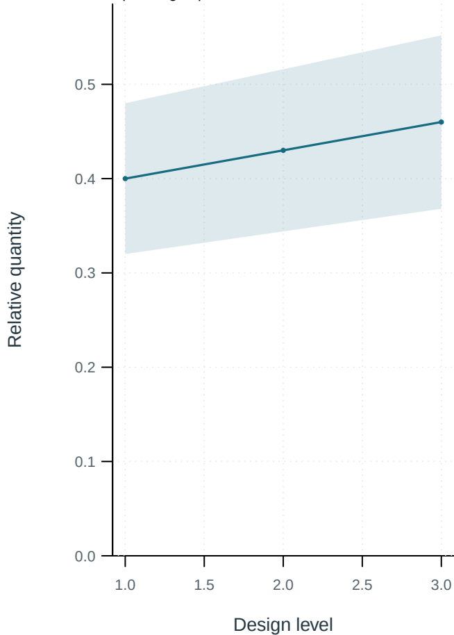
Spawning depletion
