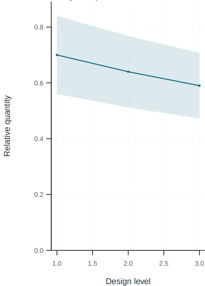
Fishing intensity
