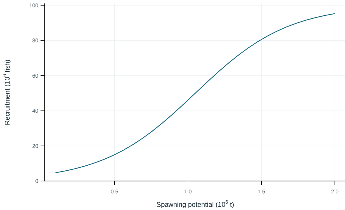
Figure 34: Illustrative output. Stock–recruitment observations and fitted relationship.
