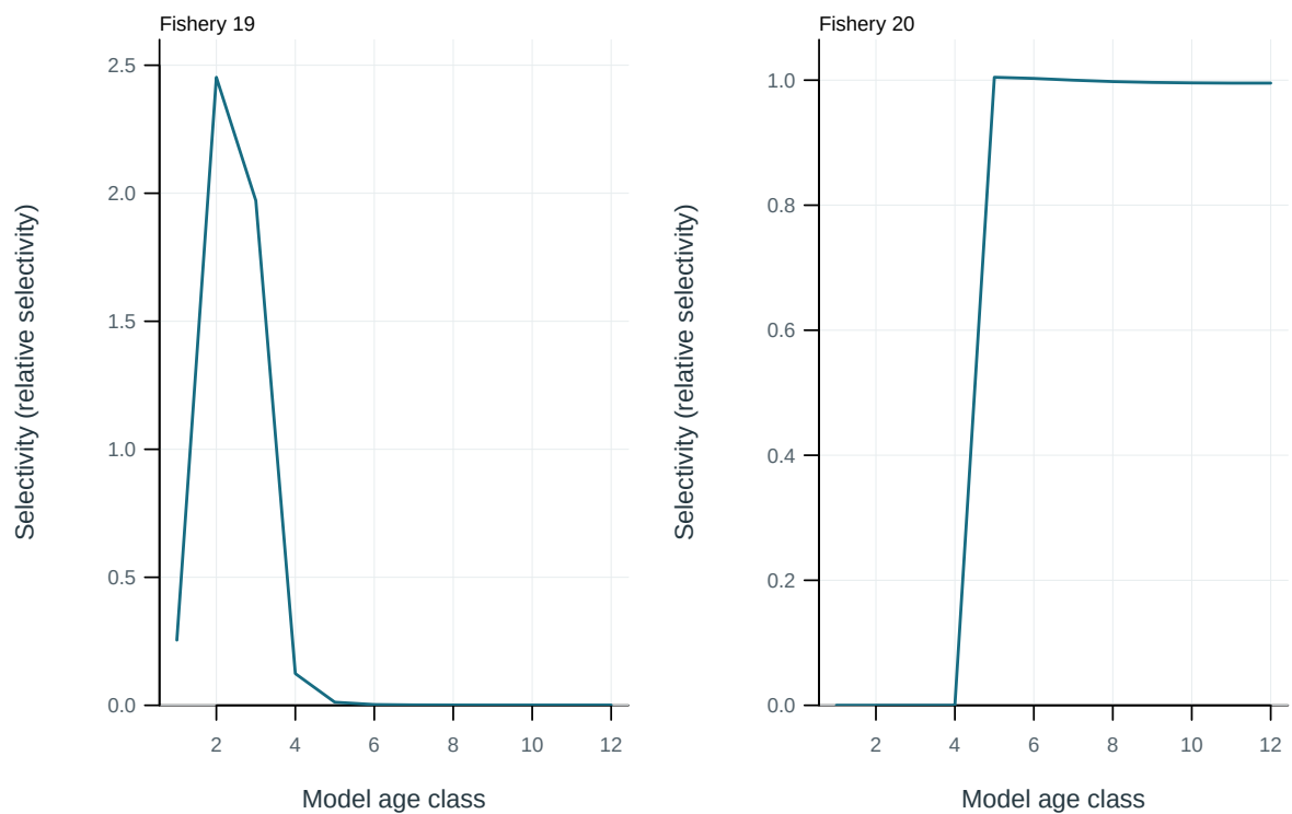
Figure 42: Fishery selectivity at age.
